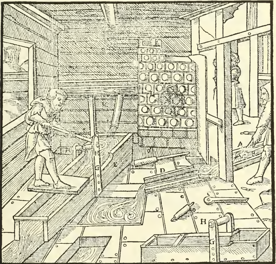
A—FIRST LAUNDER. B—THREE-TOOTHED RAKE. C—SMALL SETTling PIT. D—LARGE BUDDLE. E—BUDDLE RESEMBLING THE SIMPLE BUDDLE. F—SMALL ROLLER G—BOARDS. H—THEIR HOLES. I—SHOVEL. K—BUILDING. L—STOVE. (THIS PICTURE DOES NOT ENTIRELY AGREE WITH THE TEXT).
